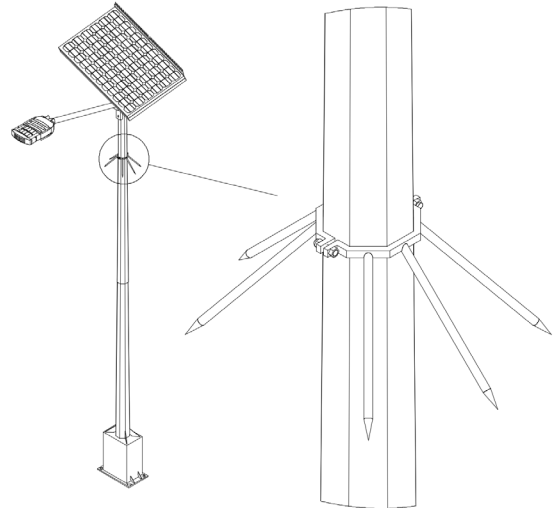
ANTI-CLIMBING SPIKES
